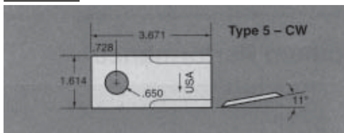
PART NO. CUT 05913
