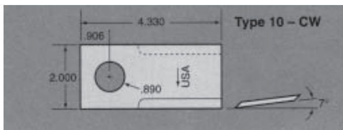
PART NO. CUT 05925
