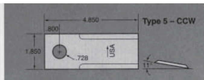
PART NO. CUT 05926
