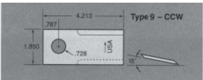
PART NO. CUT 05945
