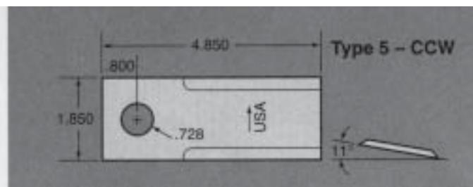
PART NO. CUT 05910
