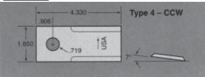
PART NO. CUT 05912
