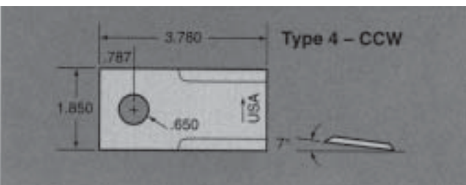
PART NO. CUT 05908
