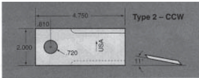
PART NO. CUT 05910
