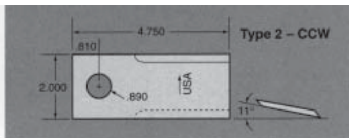
PART NO. CUT 05928
