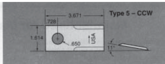
PART NO. CUT 05943
