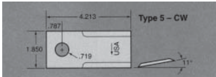
PART NO. CUT 05942
