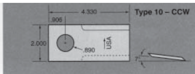
PART NO. CUT 05926
