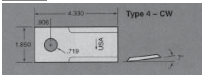
PART NO. CUT 05911
