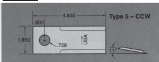
PART NO. CUT 05908
