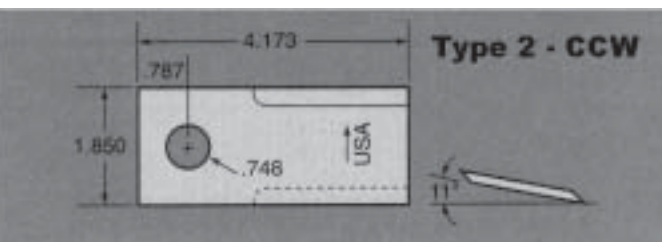
PART NO. CUT 05936
