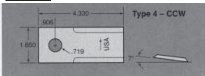
PART NO. CUT 05910
